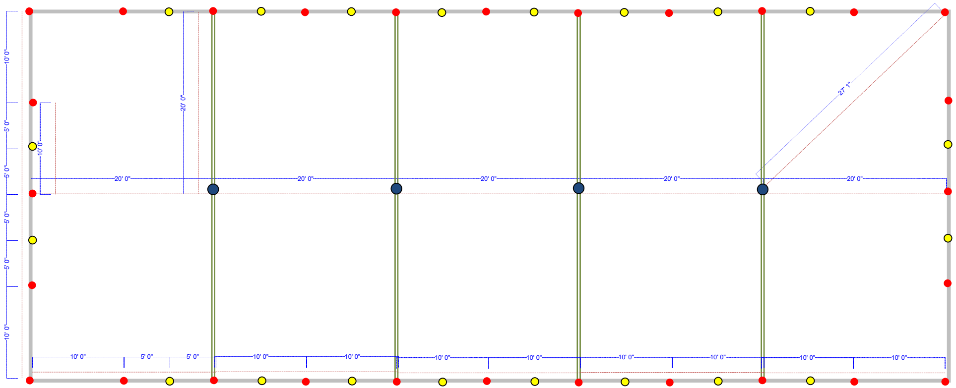
40' x 100' Pole Tent Standard & Wind - Pole Placements
